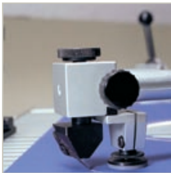
45°/90° cutting head
